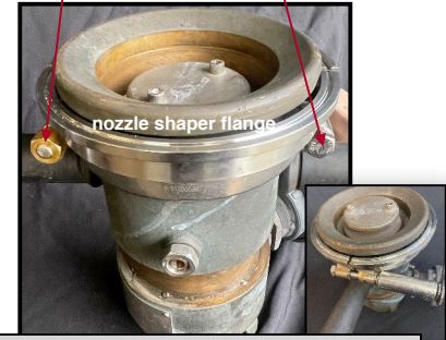
Tighten nuts evenly, just enough to flatten lock washers. Use 5/8" socket. DO NOT USE IMPACT WRENCH
