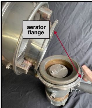
Attach nozzle flange to aerator flange. Capture both with hinged mounting collar. Snug tight thumb screw. If permanent, use blue lock tight on thumb screw threads.
